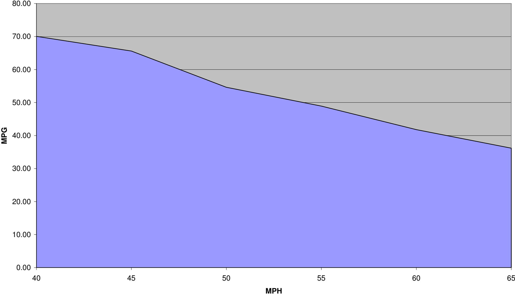
T4 Syncro Speed V Fuel Consumption
